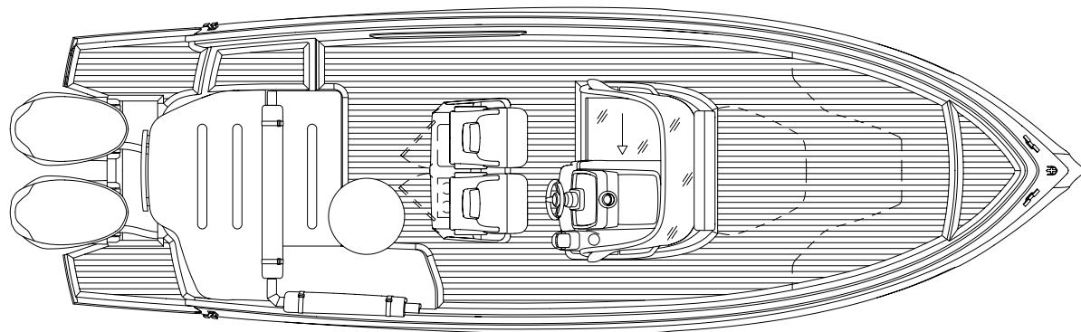
MAIN DECK
