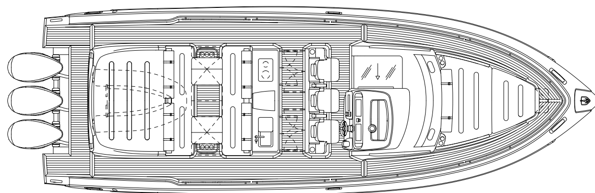
MAIN DECK
