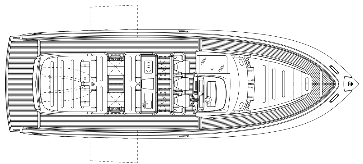
MAIN DECK
